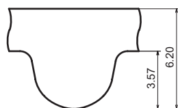
Belt tooth pitch 8mm
